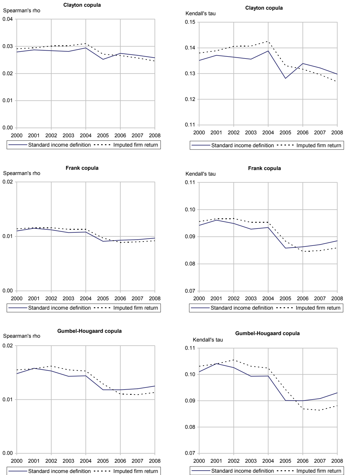
Figure 1. HI estimates for Norway 2000–2008 based on copula estimation: Clayton, Frank and Gumbel-Hougaard copulas
