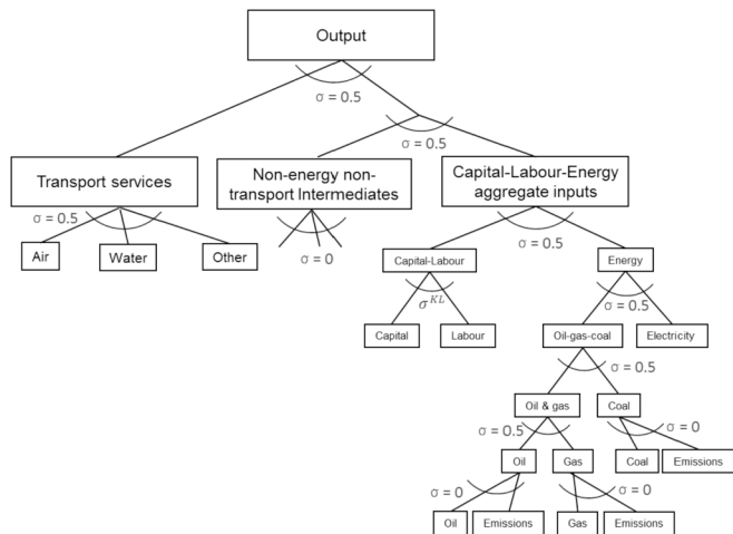
Fig. 4. Nested CES structure of production technology for non-fossil fuel extraction industries.
