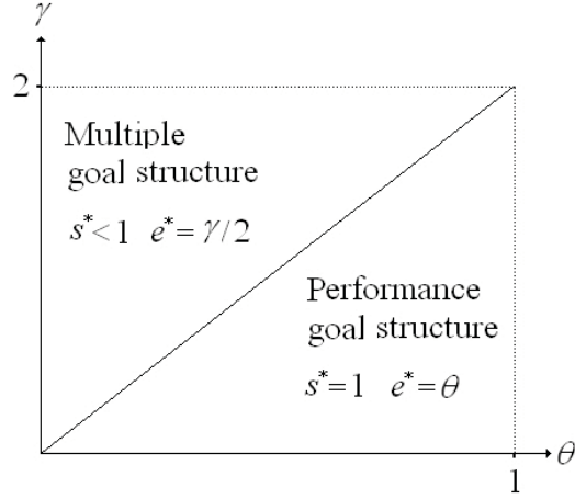
Figure 2: Equilibria in the static framework
