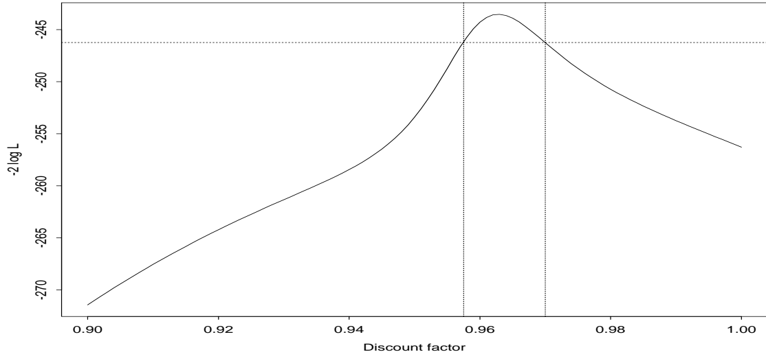
Figure 1: Plot of -2 \log -likelihood for discount factor \delta varying in [0.9, 1.0] .
